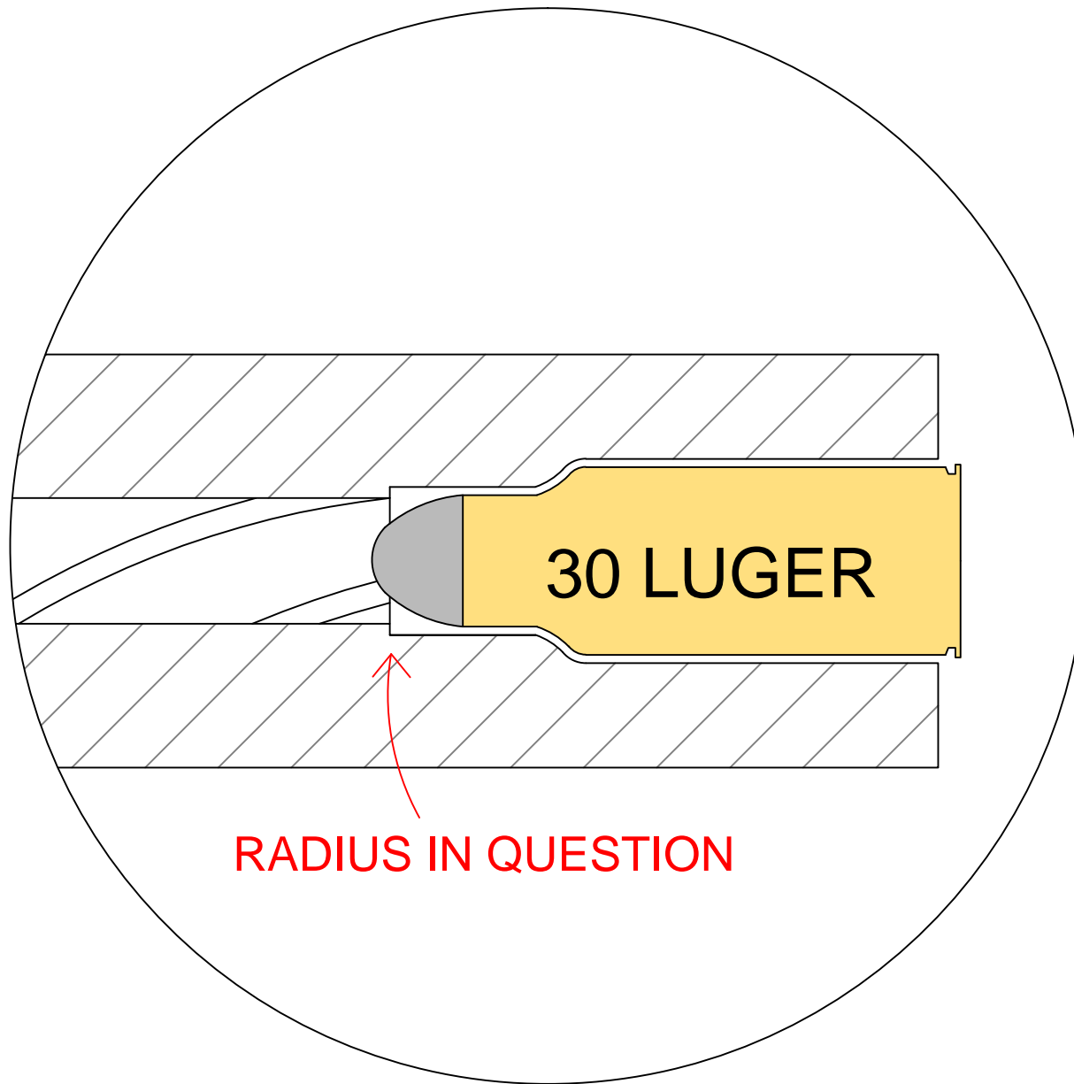
BARREL SECTION VIEW AT CHAMBER END.
